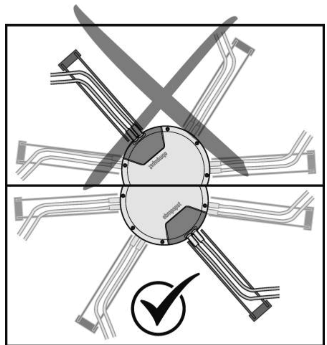
Fig. 2: Cable routing for fans installed upright.
