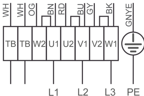
High speed/D-connection
