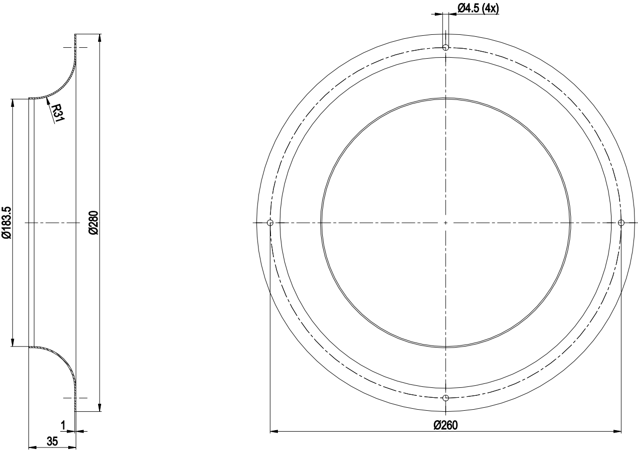
Inlet ring 96360-2-4013
