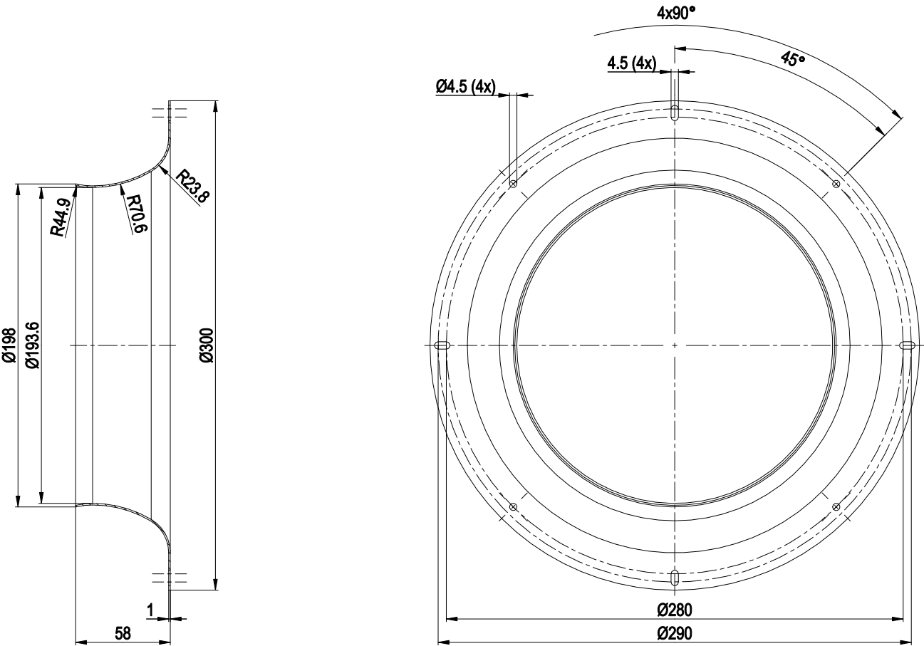
Inlet ring 31000-2-4013
